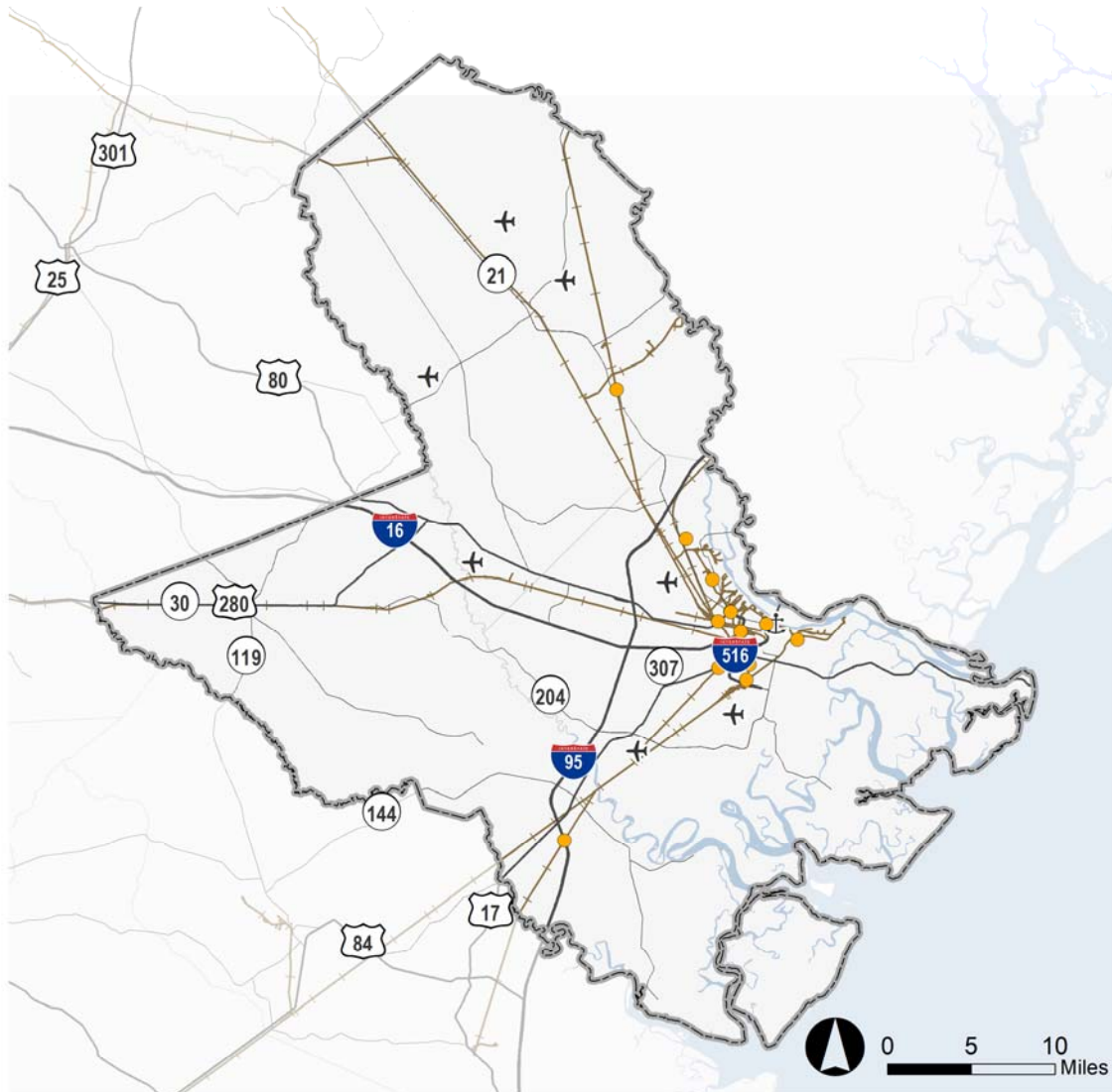
FIGURE 3.3 VERTICAL UNDERCLEARANCE ISSUES ON BRIDGES OVER RAILROADS, 2022
